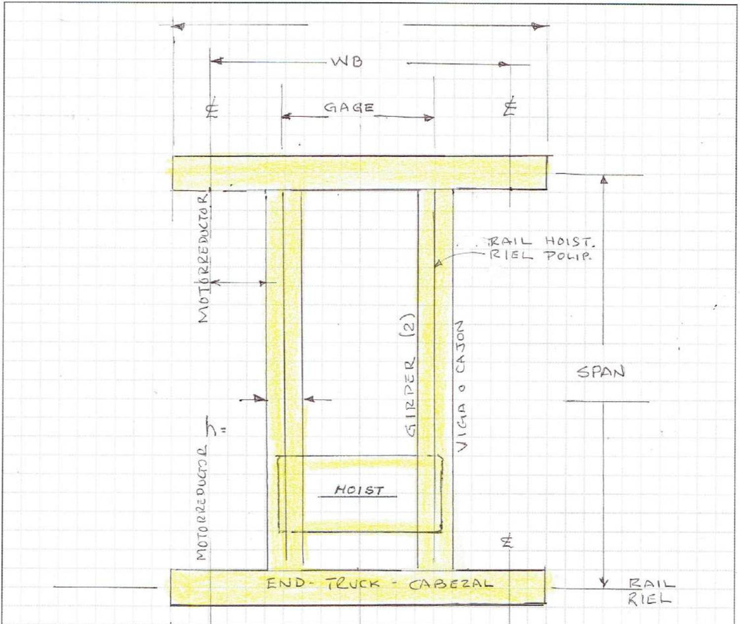
DOUBLE GIRDER CRANE - LAY-OUT - GRUA BIRRIEL.
