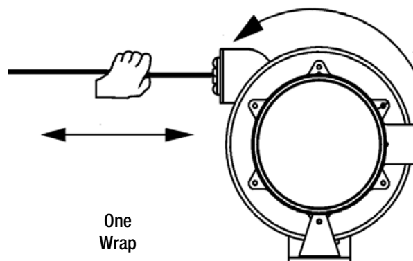
Adding Spring Tension
