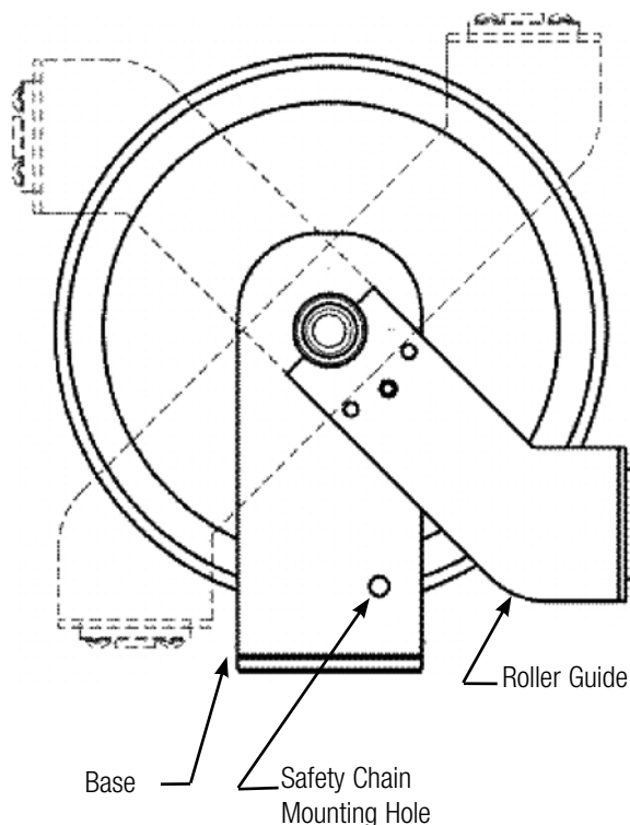
Roller Guide Locations (4 of 12 possible positions shown)
