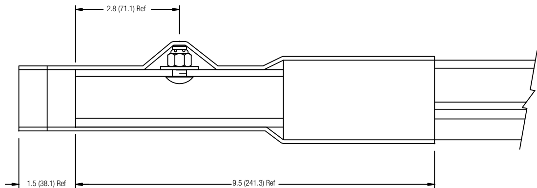
1000A End Cover (33796B)
