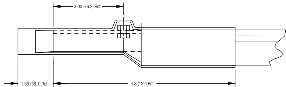
700A End Cover (50859)
