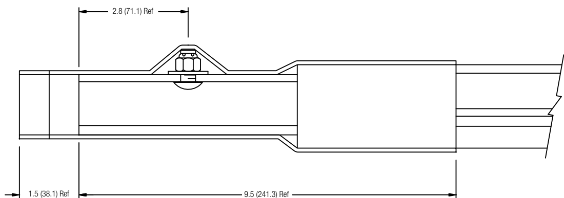
1500A End Cover (33796B)
