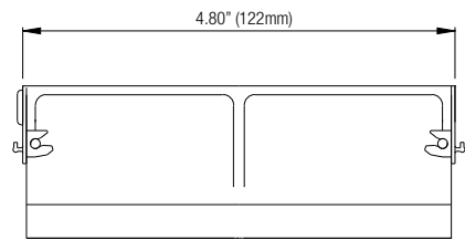
Standard Phase Cover (310850B)
